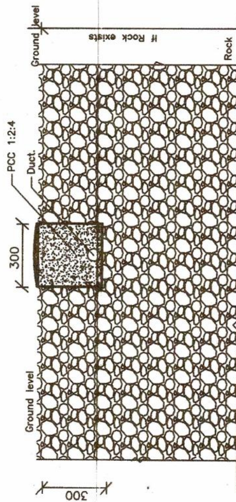
FIG.3.3 AFTER COMPLETION OF WORK.
