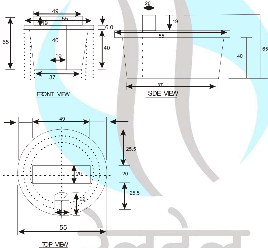
Figure 3 Rubber Cork
