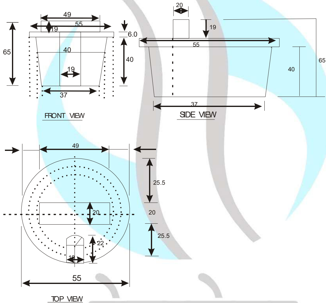
Figure 3 Rubber Cork
