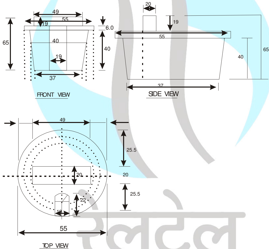
Figure 3 Rubber Cork
