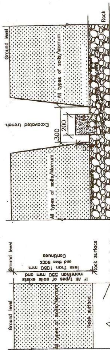
FIG.5.1 SOIL STRATA. DURING EXECUTION OF WORK.
